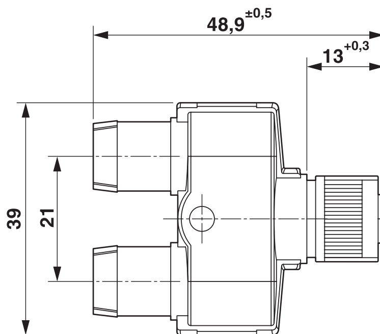
Dimensional drawing
