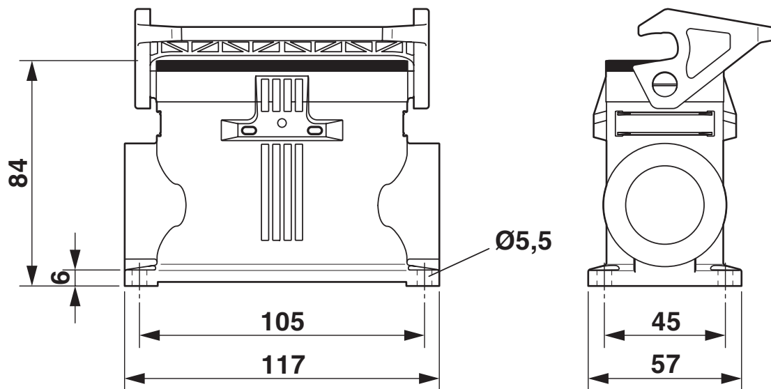
Dimensional drawing
