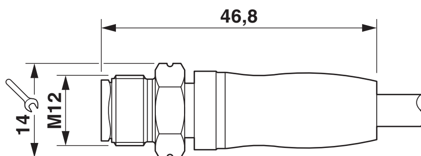
Dimensional drawing
