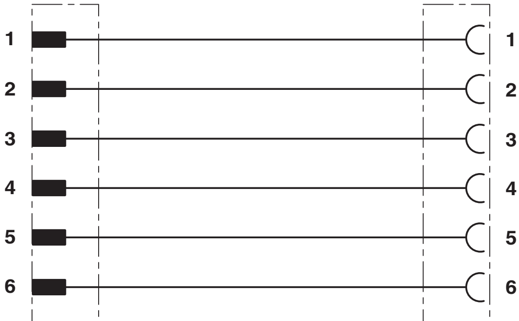
Circuit diagram
