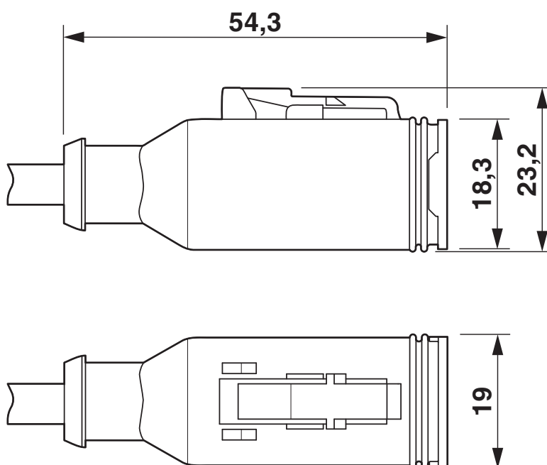
Dimensional drawing
