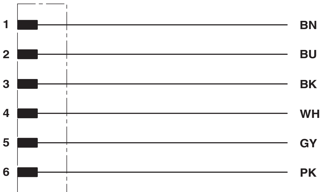
Circuit diagram
