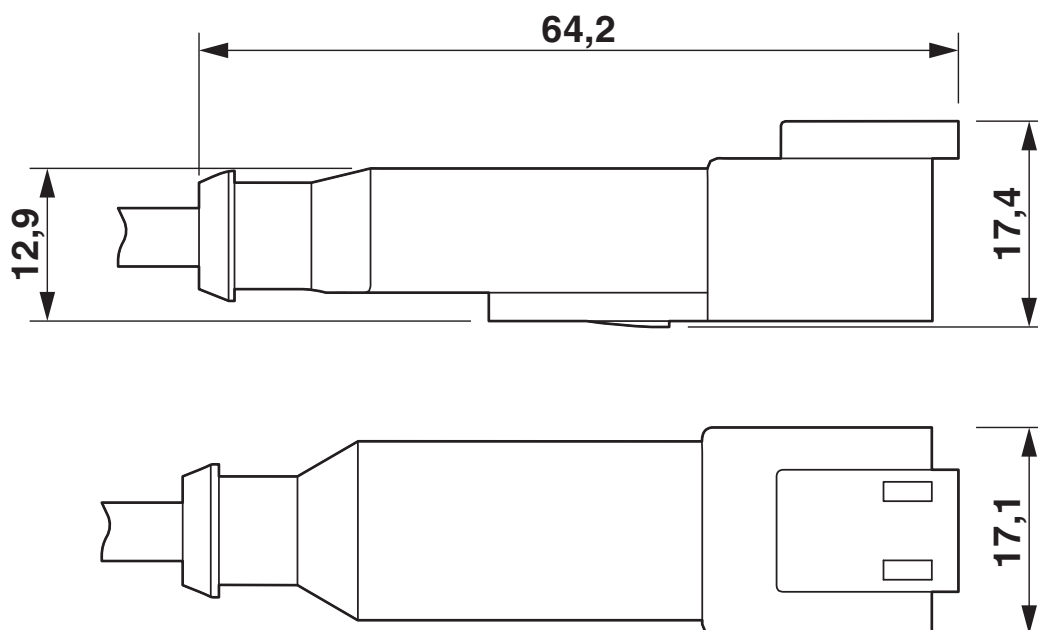
DEUTSCH DT04-2P, top view and side view
