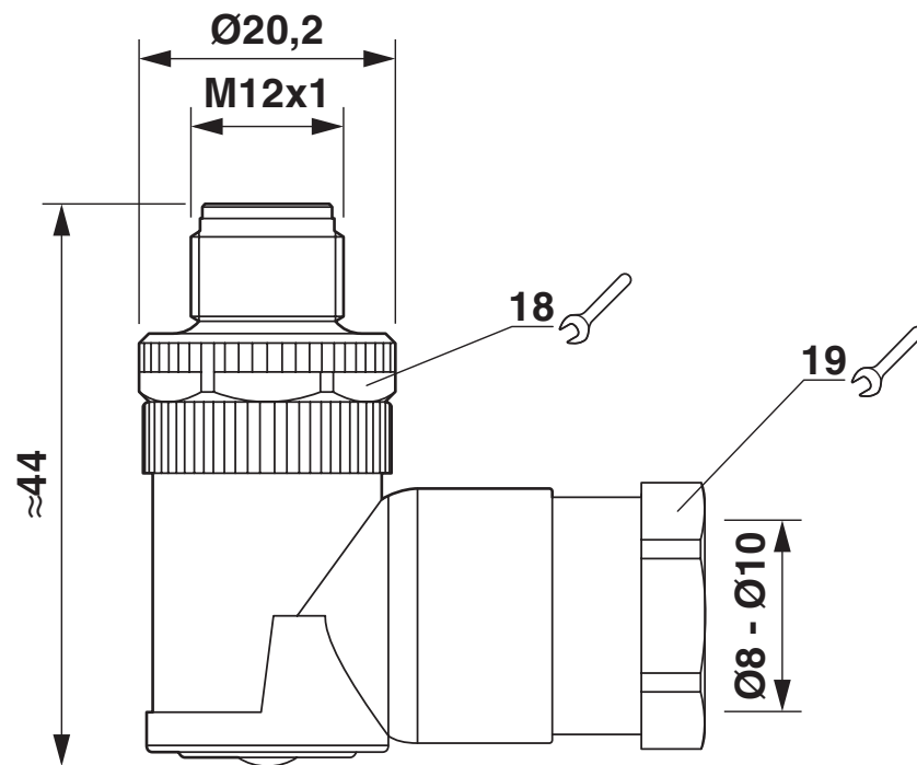
Dimensional drawing
