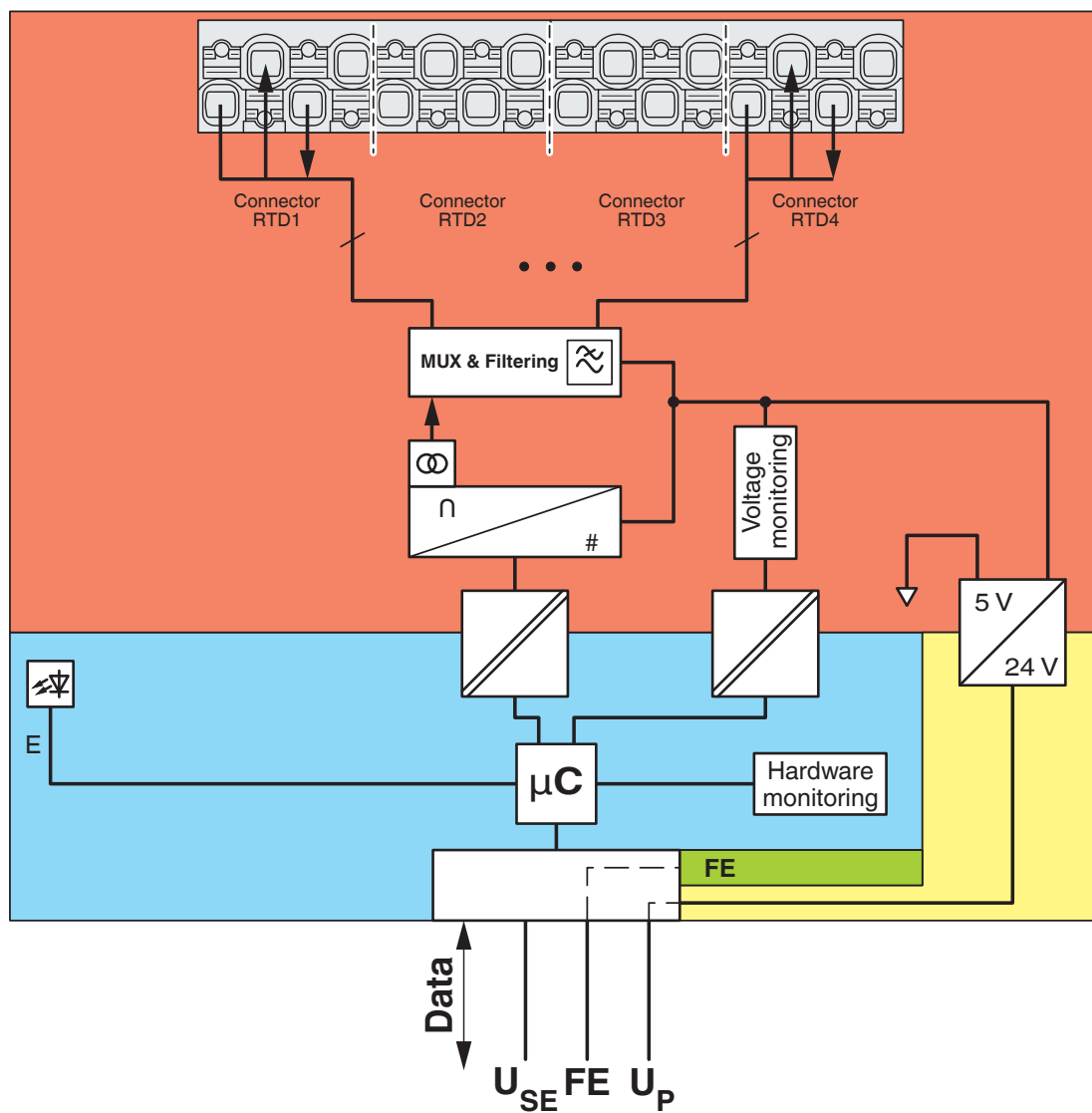
Block diagram
