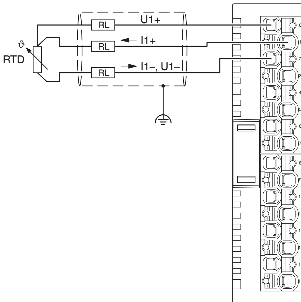
Connection diagram
