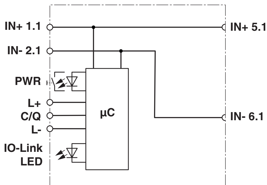
Block diagram
