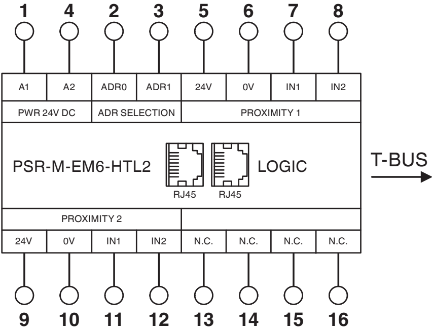
Block diagram
