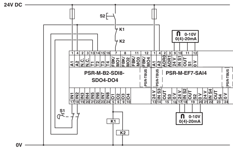
Application drawing
