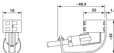
Locking clip mounted on angled M12 connector (not supplied as standard)
