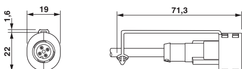
Locking clip mounted on straight M12 connector (not supplied as standard)
