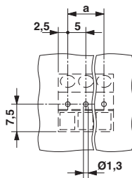
Drilling diagram
