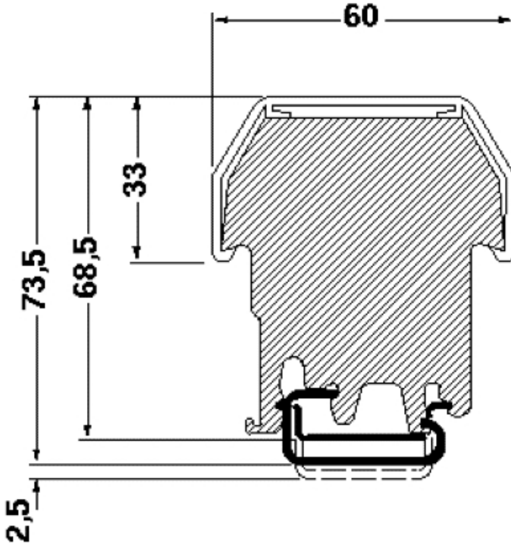
Dimensional drawing
