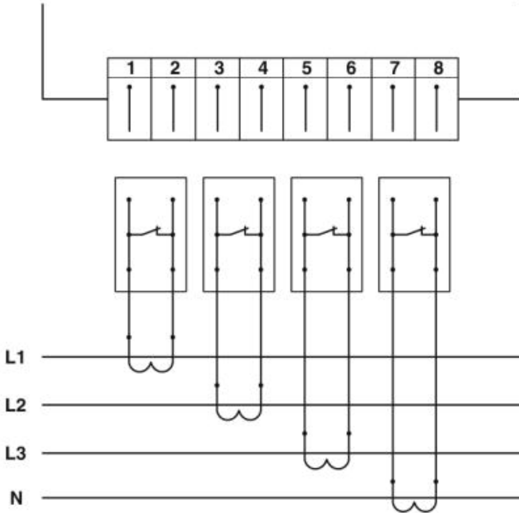
Circuit diagram
