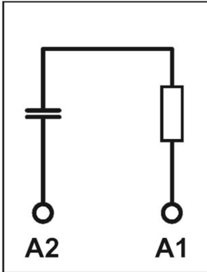
Circuit diagram
