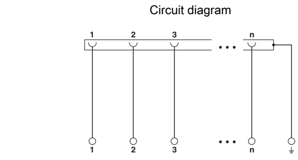
Universal circuit diagram
