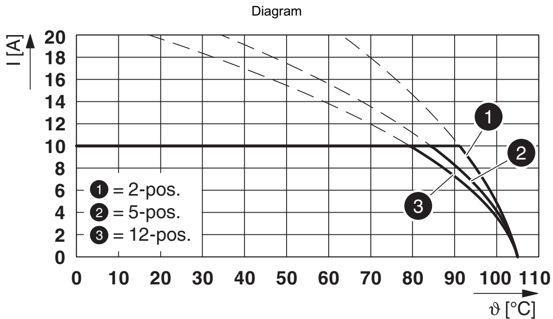
Type: FKCVW 2,5/...-STF with MDSTB 2,5/...-GF
