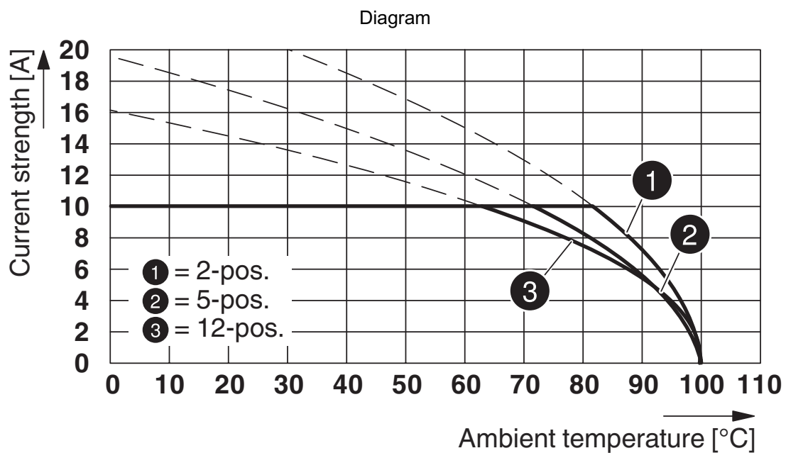
Type: MSTB 2,5/...-STF with MDSTB 2,5/...-GF
