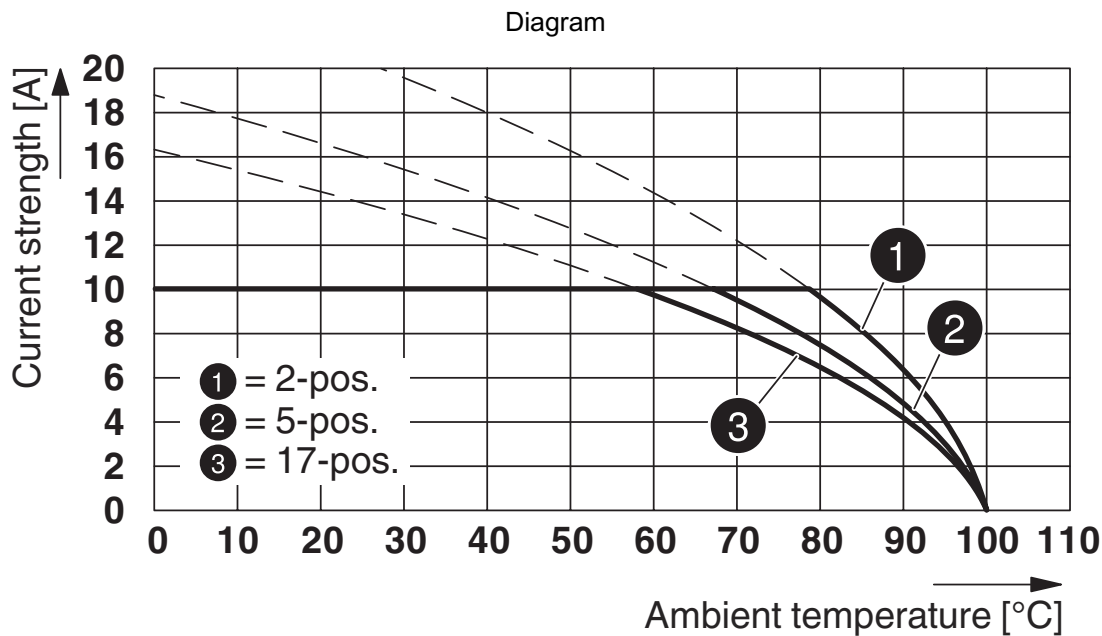
Type: FRONT-MSTB 2,5/...-STF-5,08 with MDSTB 2,5/...-GF-5,08
