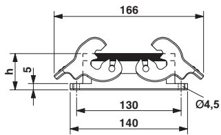
Dimensional drawing
