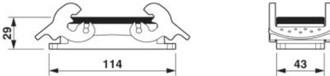
Dimensional drawing
