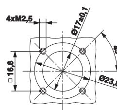
Dimensional drawing
