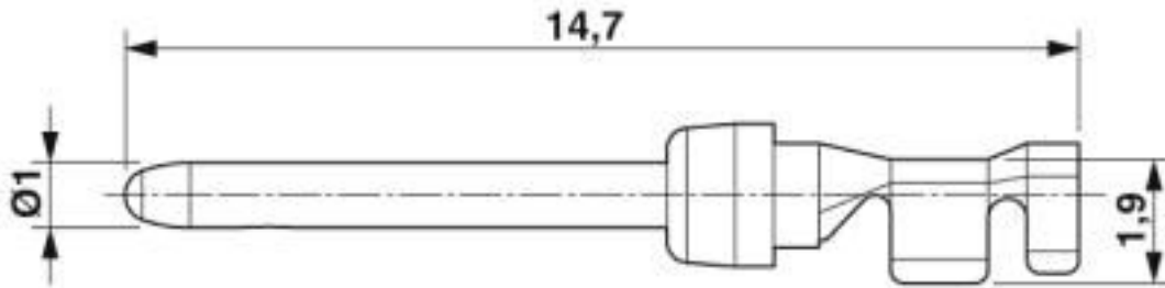
Dimensional drawing
