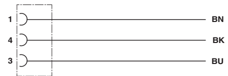
Contact assignment of the M 8 sockets, 3-pos.
