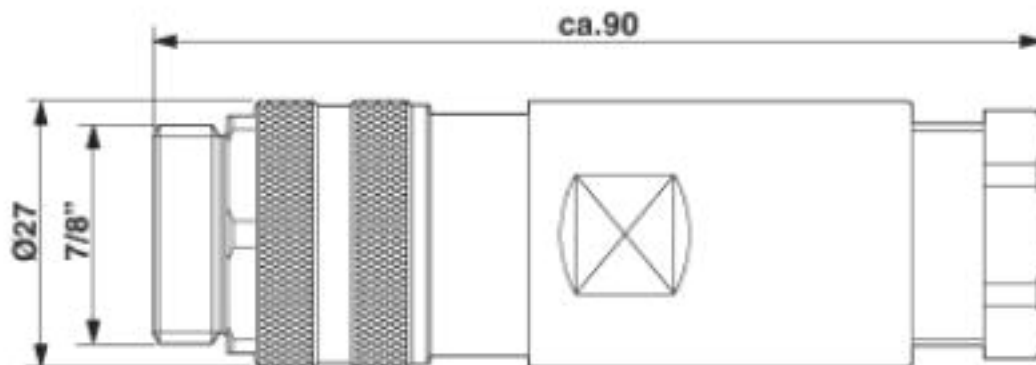
Dimensional drawing
