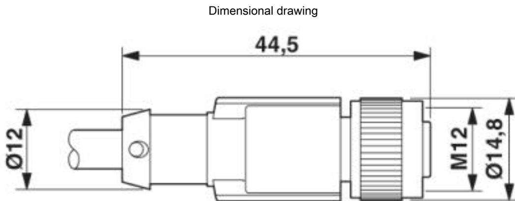
M12 x 1 socket, straight, shielded
