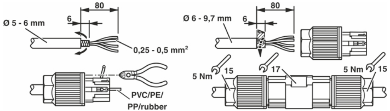
Functional drawing
