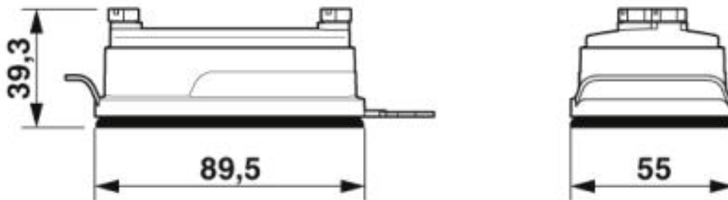
Dimensional drawing
