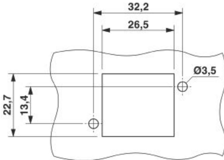
Dimensional drawing
