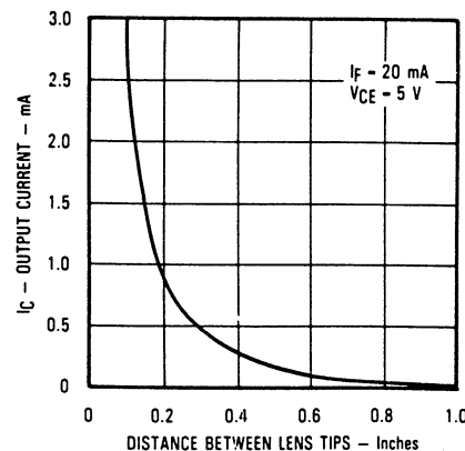
Coupling Characteristics of OP168F and OP508F
