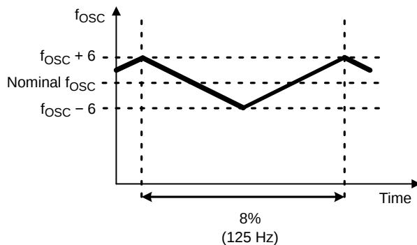
Figure 34. Frequency Jittering
