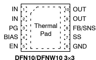
DFN10/DFNW10 3x3
