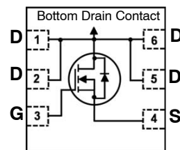
Single N-Channel MOSFET
