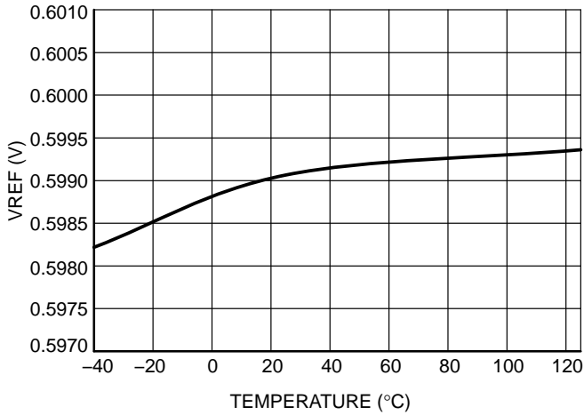
Figure 10. V_{\text{REF}} vs T at V_{\text{HVBIA}} = 48\text{ V}
