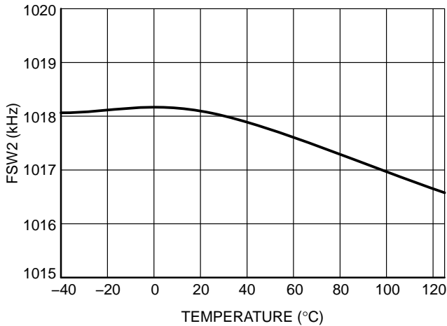
Figure 14. Switching Frequency vs. T at V_{\text{HVBIA}} = 48\text{ V} and R_T = 8.06\text{ k}\Omega
