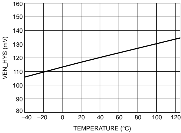
Figure 12. EN/UVLO Hysteresis Voltage vs. T at V_{\text{HVBIA}} = 48\text{ V}
