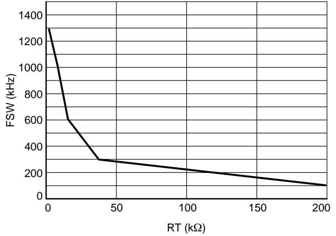
Figure 13. Switching Frequency vs. R_T at V_{\text{HVBIA}} = 48\text{ V} and T = 25^\circ\text{C}
