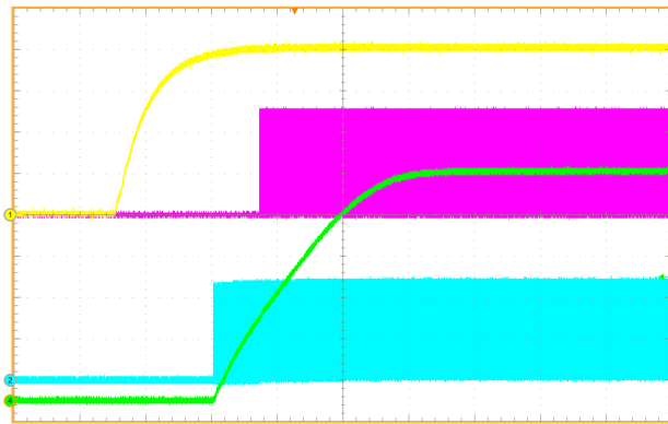
CH1 = EN (0.5V/div), CH2 = SW (20V/div), CH3 = LG (2V/div), CH4 = Vo (5V/div), T = 2mS/Div
