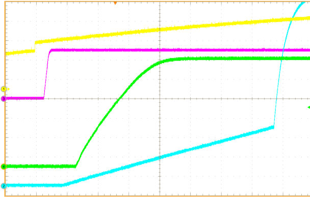
CH1 = EN (0.5V/div), CH2 = SS (0.5V/div), CH3 = Vcc (2V/div), CH4 = Vo (5V/div), T = 2mS/Div
