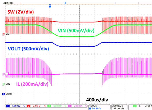
Figure 28. Pass Thru Operation, I_{OUT} = 10\text{ mA} , V_{IN} = 3 \leftrightarrow 2.4\text{ V} , V_{OUT} = 2.6\text{ V}
