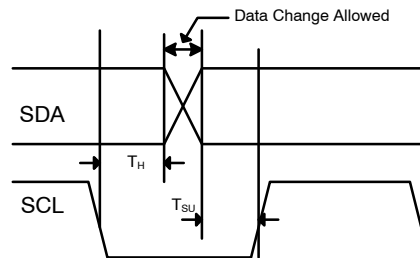
Figure 35. Data Transfer Timing
