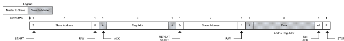
Figure 40. Single Register Read Transaction
