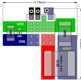
Figure 2. Reduced-Footprint Layout
