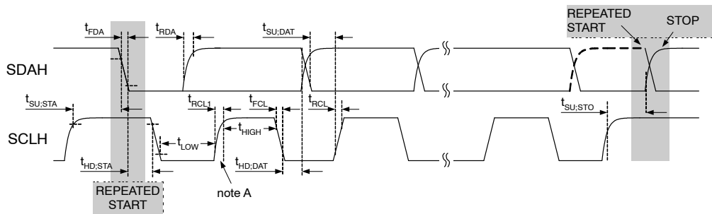
Figure 5. I 2 C Interface Timing for Fast Plus, Fast, and Slow Modes
