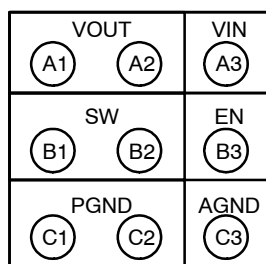
Figure 3. Top View
