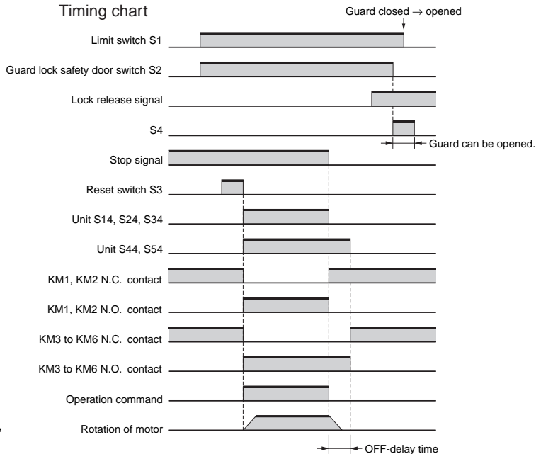
Timing chart
