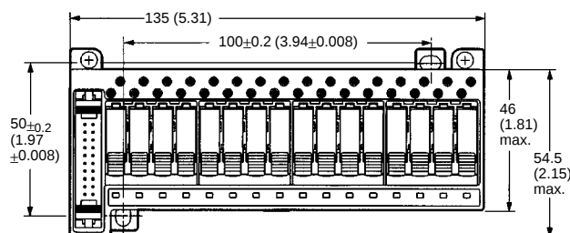
Terminal Block (with Expansion Terminal Block)
