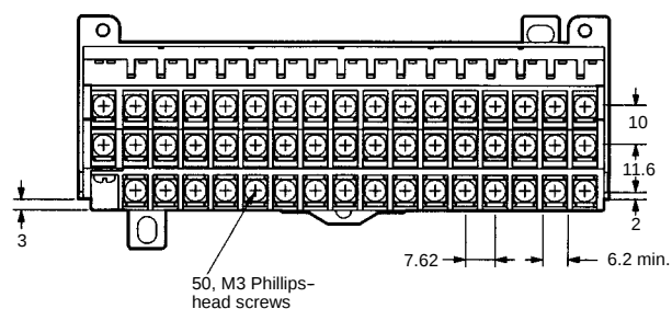
Terminal Block (with Expansion Terminal Block)
