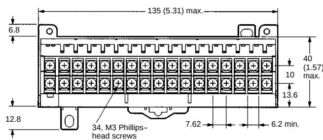
Terminal Block (without Expansion Terminal Block)
