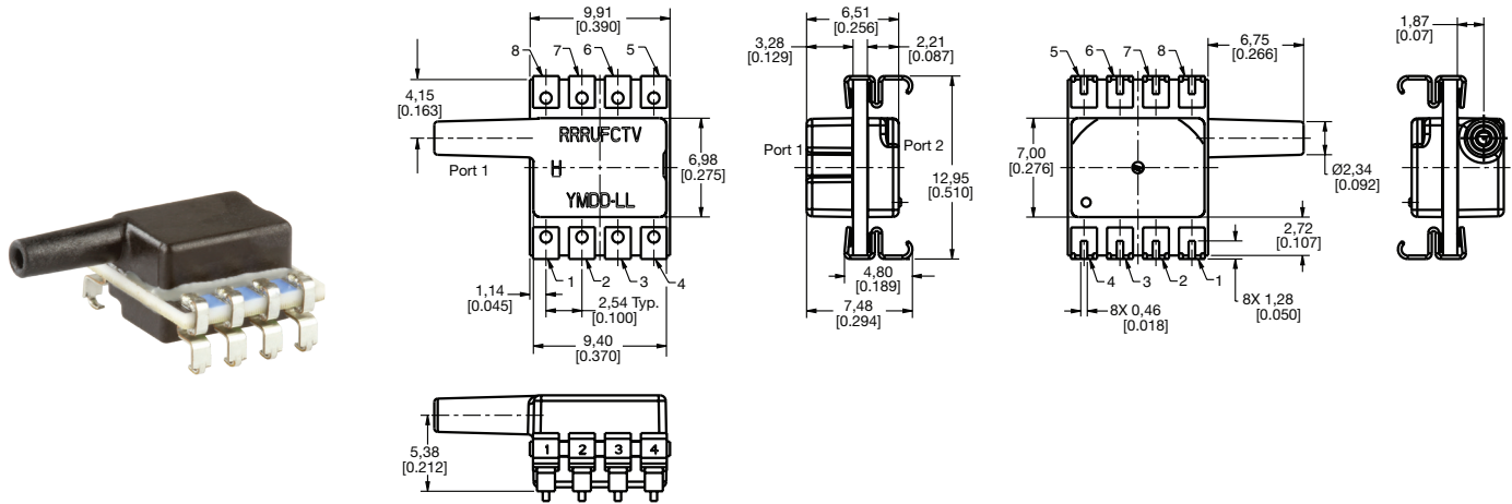
FIGURE 5. SMT PACKAGE DIMENSIONAL DRAWINGS (CONTINUED)
