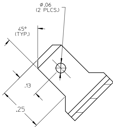
Section Z-Z
