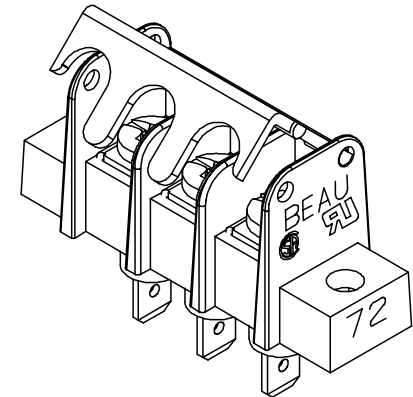
3 CIRCUIT SHOWN
