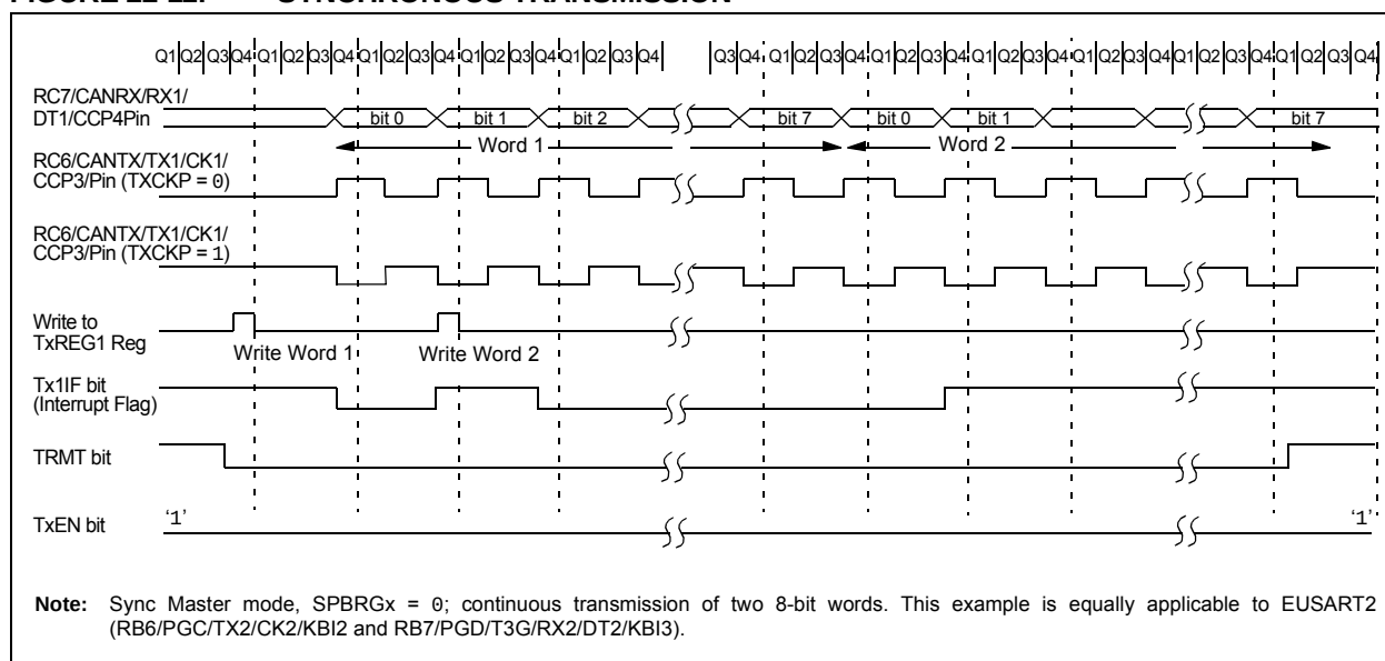
FIGURE 22-11: SYNCHRONOUS TRANSMISSION
