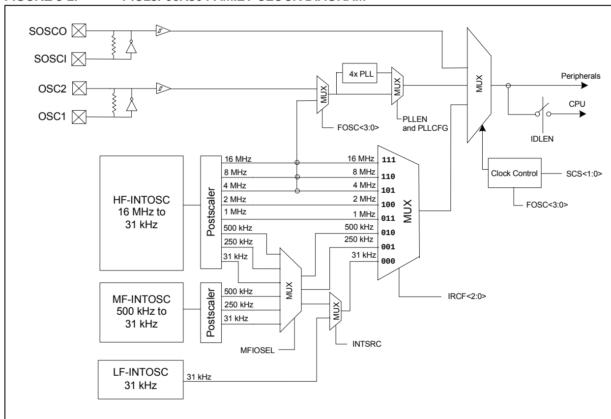
FIGURE 3-1: PIC18F66K80 FAMILY CLOCK DIAGRAM
