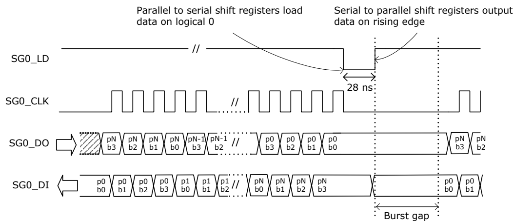
FIGURE 3-26: SIO TIMING
