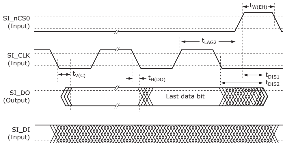
FIGURE 6-5: SI OUTPUT DATA TIMING DIAGRAM FOR SLAVE MODE
