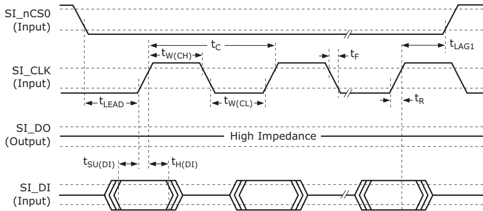
FIGURE 6-4: SI INPUT DATA TIMING DIAGRAM FOR SLAVE MODE
