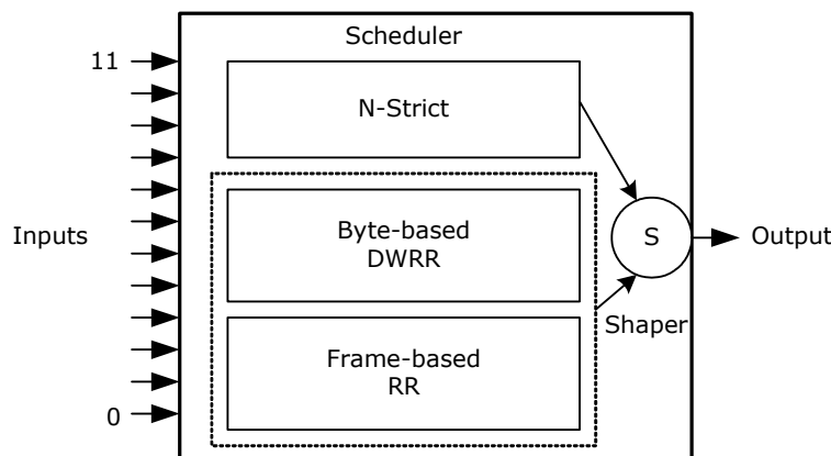
FIGURE 2-35: SCHEDULER ELEMENT
