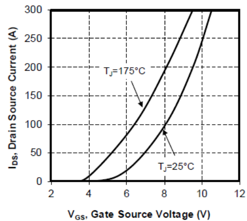
Figure 7 • Transfer Characteristics
