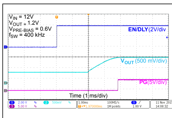
FIGURE 2-22: Enable Start-Up with Pre-Biased Output.
