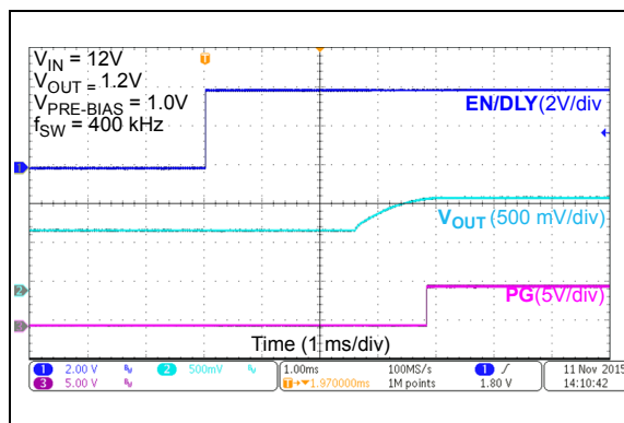
FIGURE 2-23: Enable Start-Up with Pre-Biased Output.
