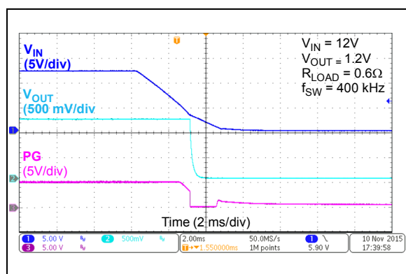
FIGURE 2-19: V_{IN} Turn-Off.
