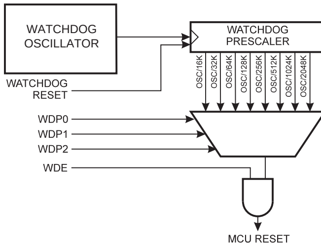
Figure 28. Watchdog Timer
