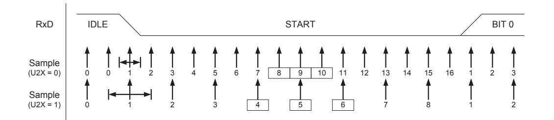
Figure 83. Start Bit Sampling
