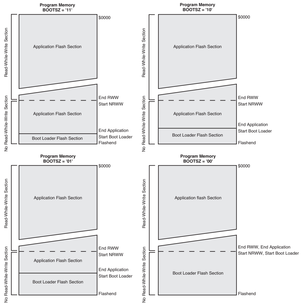
Figure 136. Memory Sections (1)
