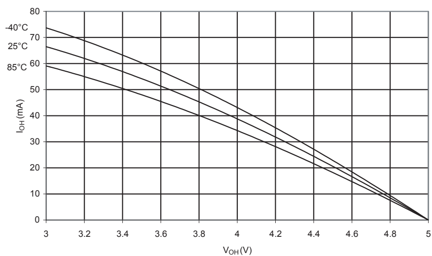
Figure 188. I/O Pin Source Current vs. Output Voltage ( V_{CC} = 5V )
