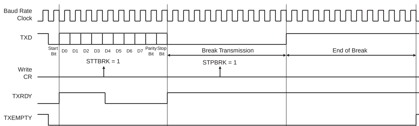
Figure 25-12. Break Transmission
