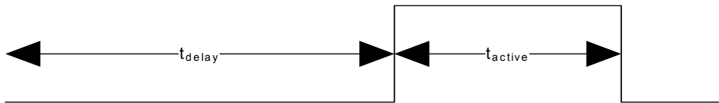
FIGURE 43-5: CPU_RESET TIMING
