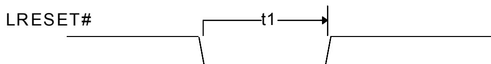
FIGURE 43-15: RESET TIMING
