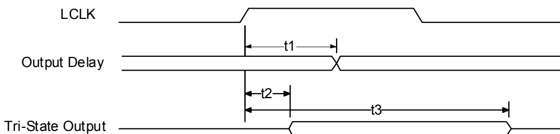
FIGURE 43-16: OUTPUT TIMING MEASUREMENT CONDITIONS, LPC SIGNALS
