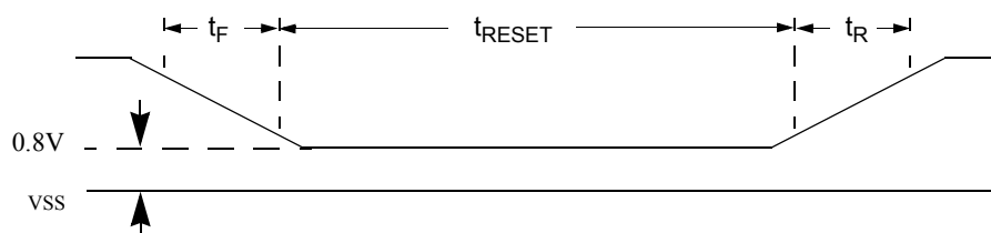
FIGURE 43-3: RESET_IN# TIMING
