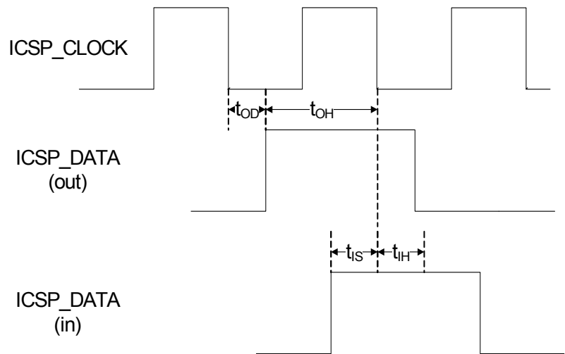
FIGURE 43-13: ICSP SETUP & HOLD PARAMETERS
